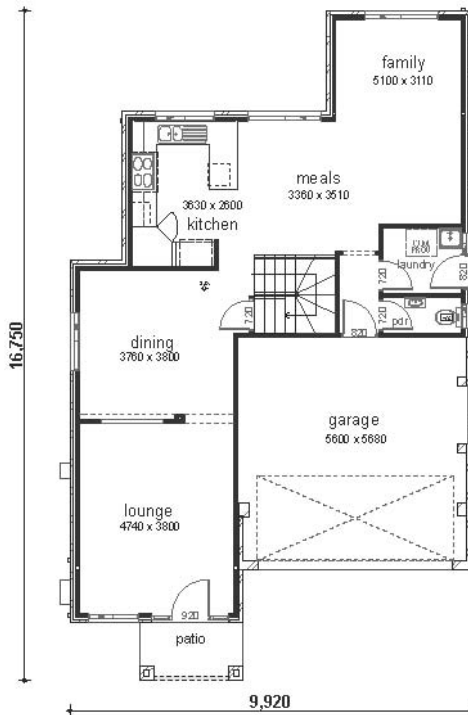
Ground Floorplan:
